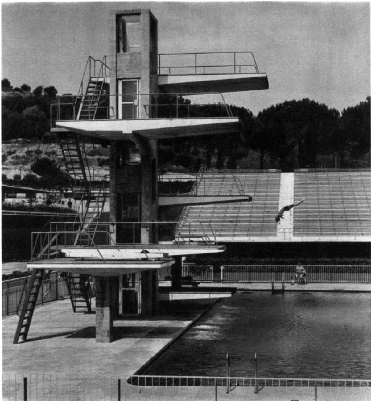
Olympic Swimming Stadium: the complex of springboards and the diving pool.
